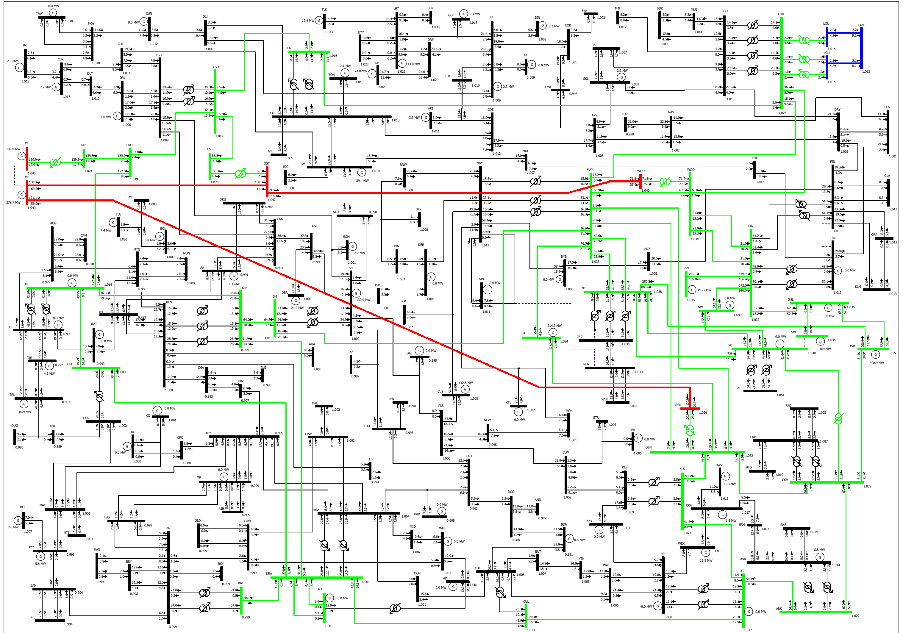
Figure J-2 Power Flow Diagram Summer Night Valley 2005
