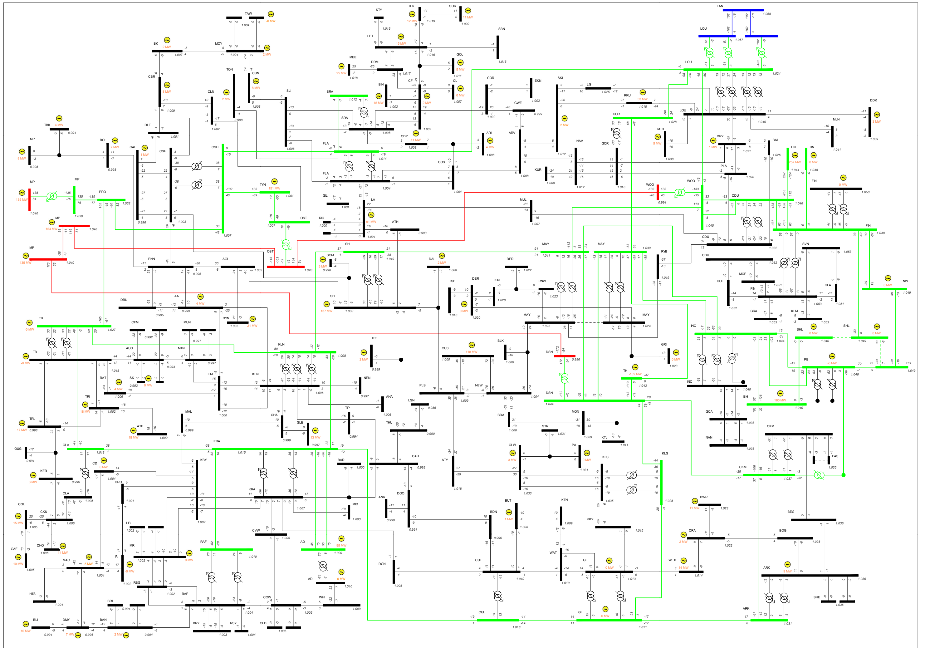
Figure J-5 Power Flow Diagram Summer Valley 2008
