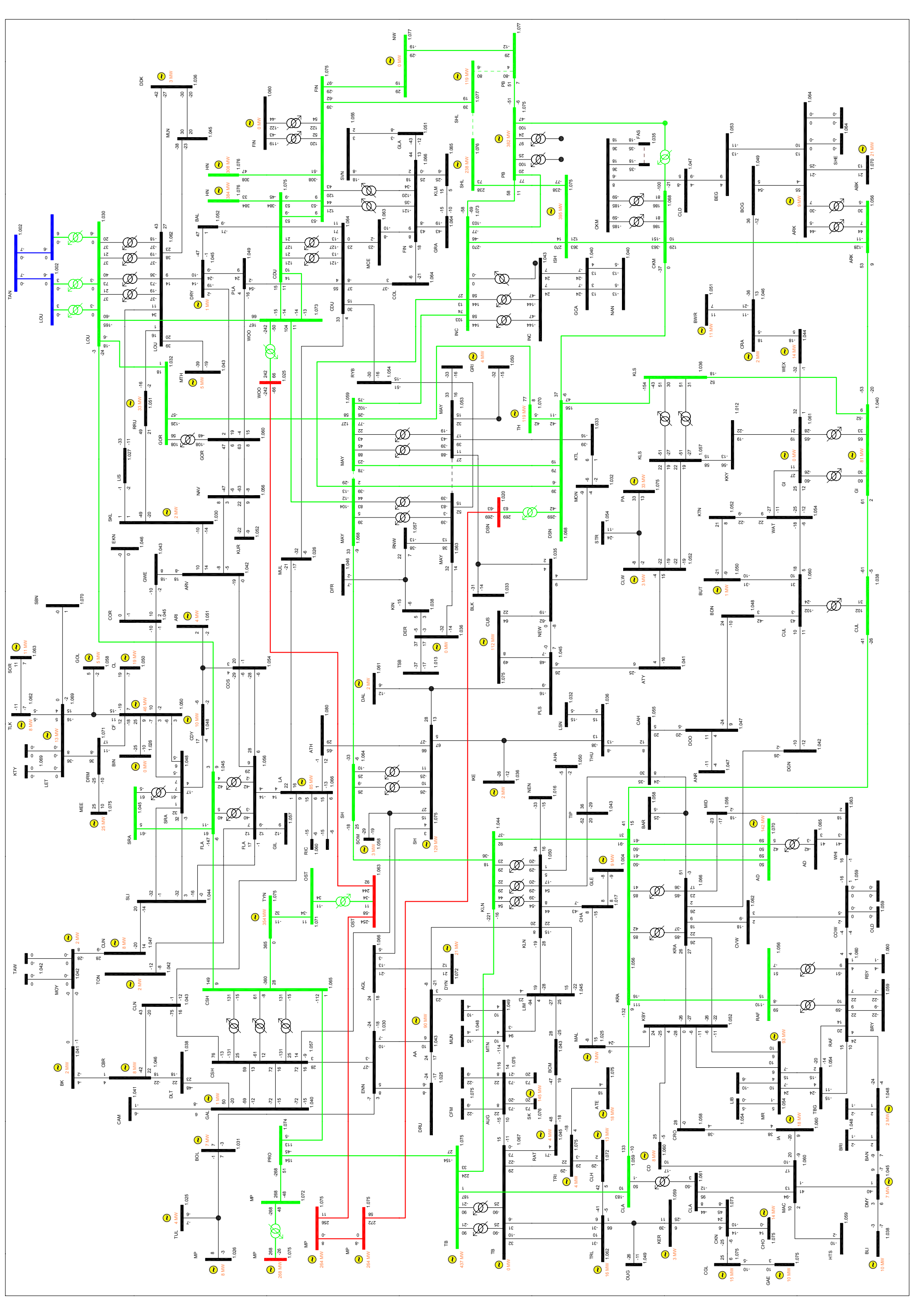
Figure J-6 Power Flow Diagram Winter Peak 2007/08
