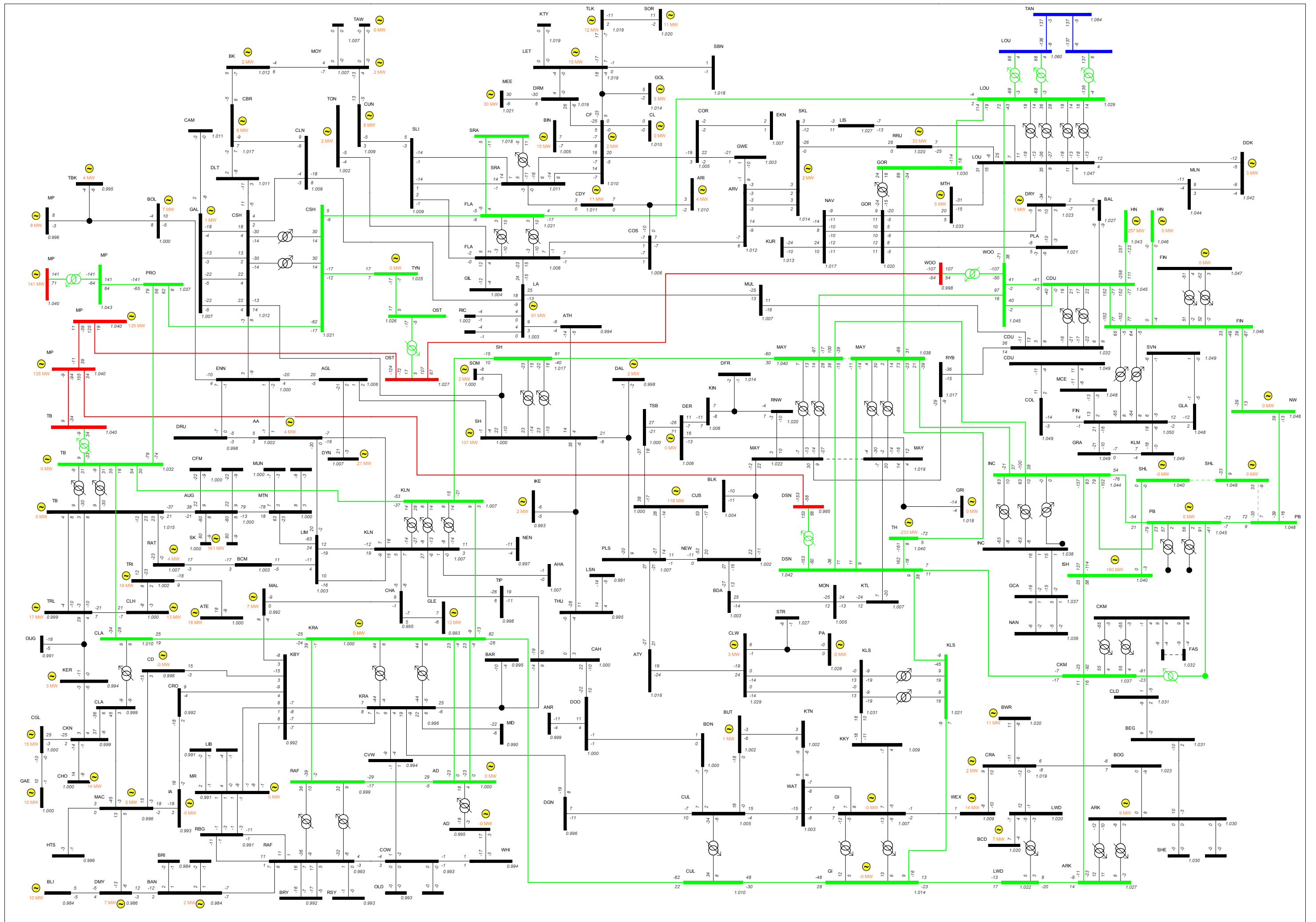
Figure J-8 Power Flow Diagram Summer Valley 2010
