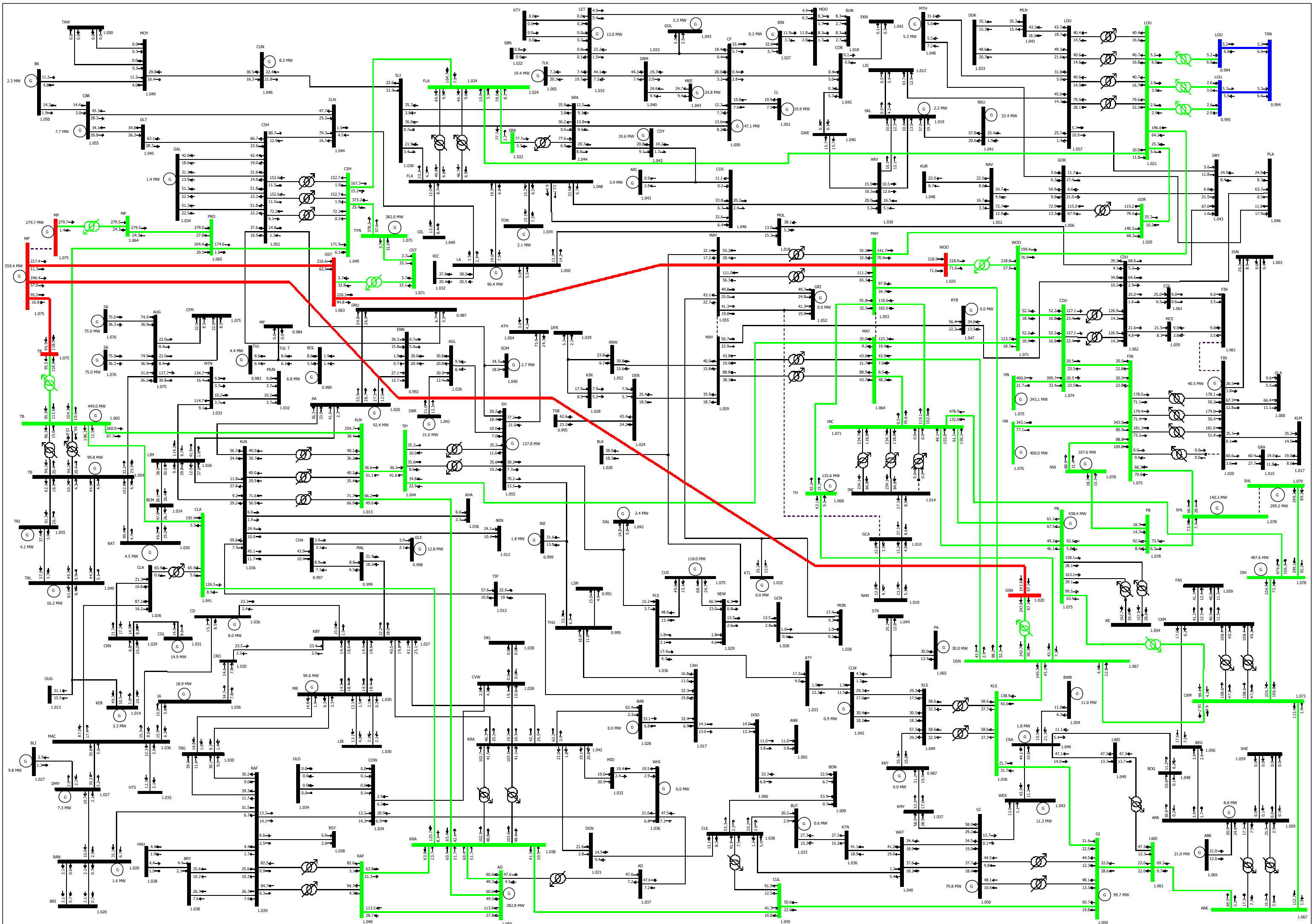
Figure J-9 Power Flow Diagram Winter Peak 2011/12
